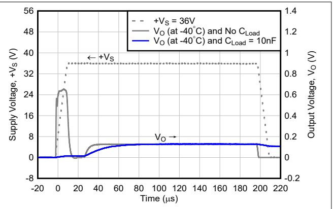
图 8-7. SR = 3.3V/\mu s 且无 C_{By-pass} 时, +V_S = 36V 阶跃的启动响应 (无 C_{Load} 且 C_{Load} = 10nF )
