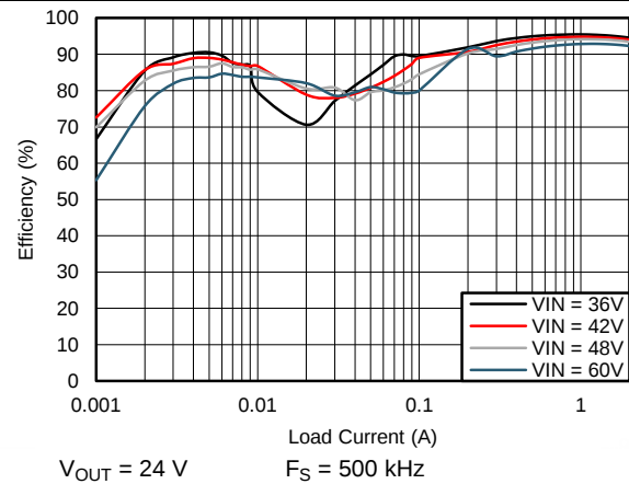
Figure 78. Efficiency
