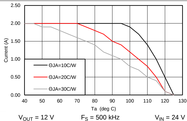
Figure 76. Derating Curve
