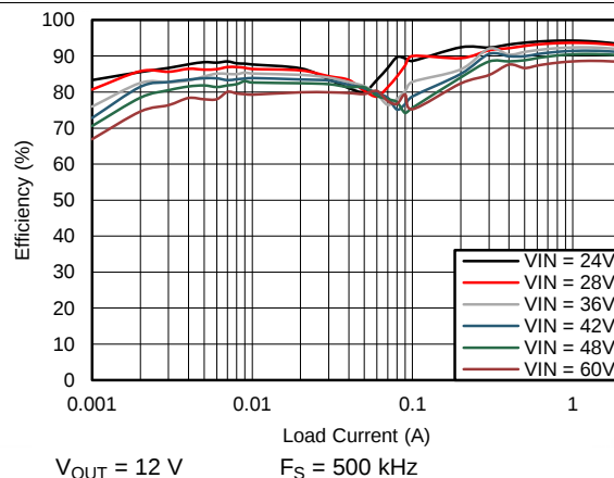
Figure 72. Efficiency
