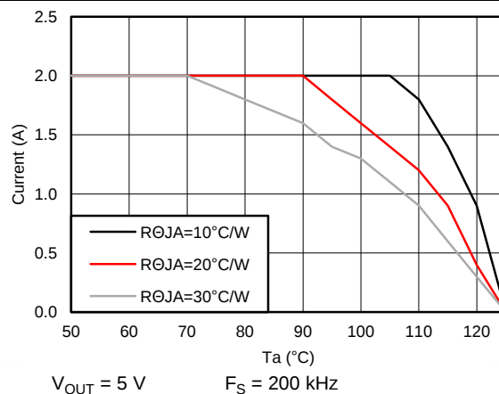
Figure 64. Derating Curve
