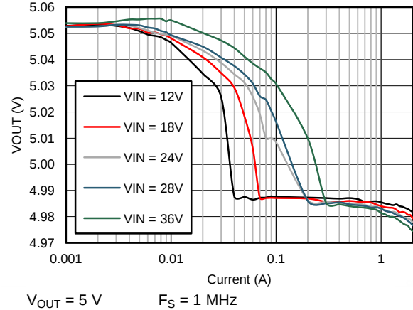
Figure 10. V_{OUT} Regulation
