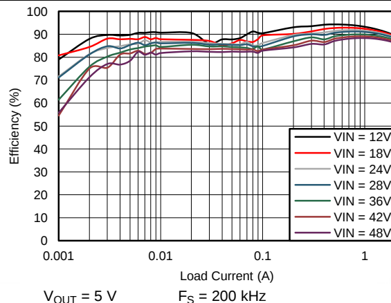
Figure 60. Efficiency
