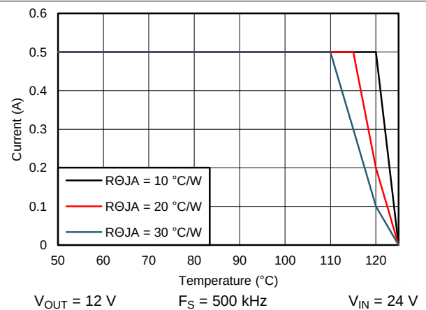
Figure 76. Derating Curve
