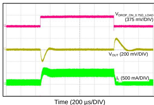
Figure 69. Load Transient Between 0.05 A and 0.5 A
