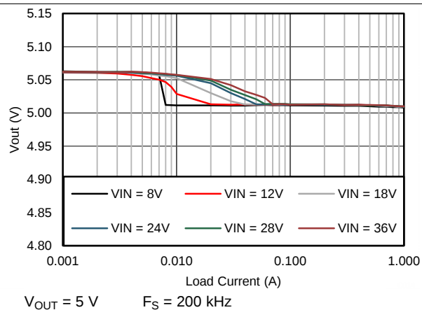
Figure 8. V_{OUT} Regulation
