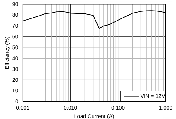
Figure 78. Efficiency
