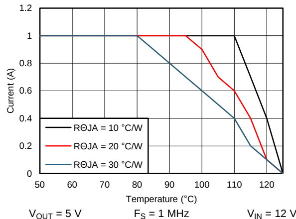
Figure 76. Derating Curve
