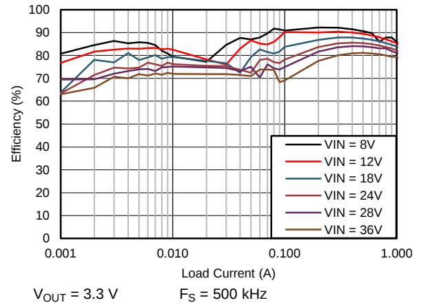
Figure 54. Efficiency
