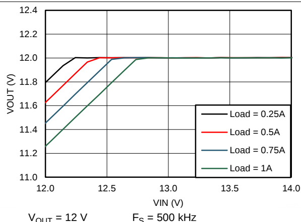
Figure 86. Dropout Curve
