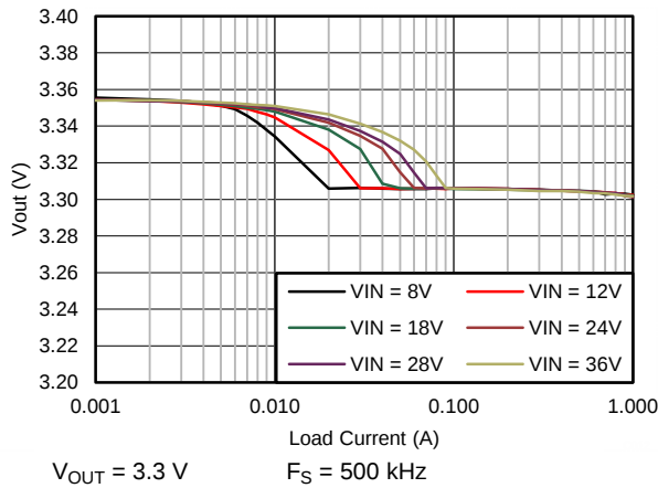
Figure 55. Output Voltage Regulation
