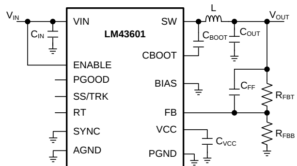
Figure 45. LM43601 Basic Schematic for V_{OUT} < 3.3 V, Tie BIAS to Ground
