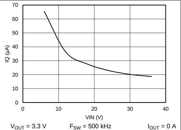
Figure 32. Operation I_Q vs V_{IN} with BIAS Connected to V_{OUT}
