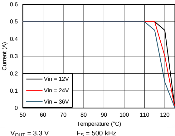
Figure 89. Derating Curve with R_{\theta JA} = 20^\circ\text{C/W}
