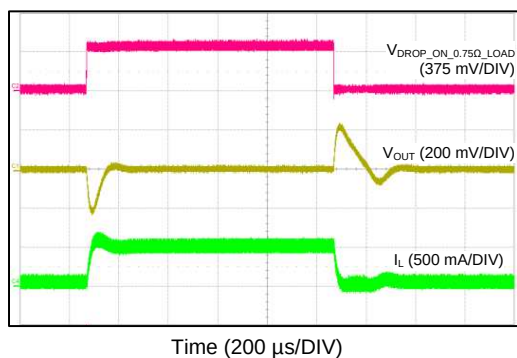
Figure 81. Load Transient Between 0.05 A and 0.5 A
