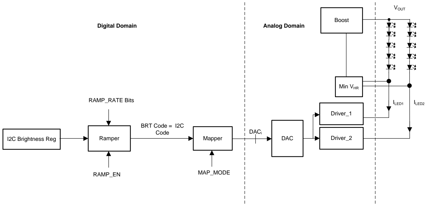
图 21. Brightness Control 00 (I²C Only)
