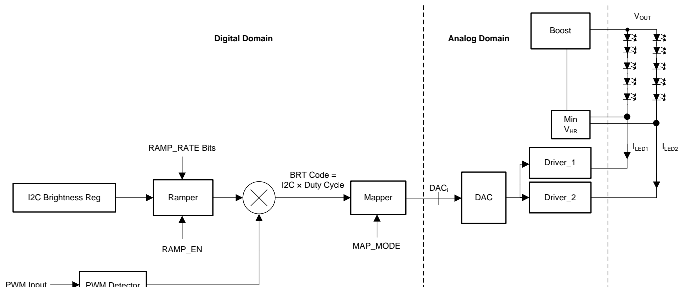
图 27. Brightness Control 11 (I²C + PWM)
