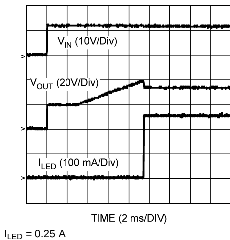
Figure 9. Power-Up Waveform
