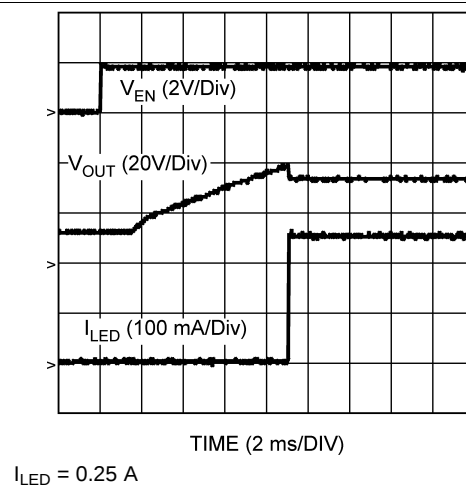
Figure 10. Enable Transient Waveform
