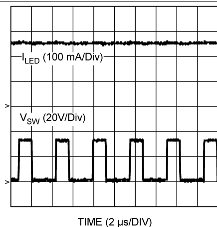
Figure 11. Steady-State Operation
