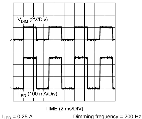
Figure 12. LED 50% Dimming Waveforms
