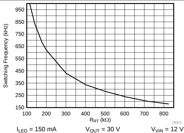
Figure 19. Switching Frequency vs RT Resistance
