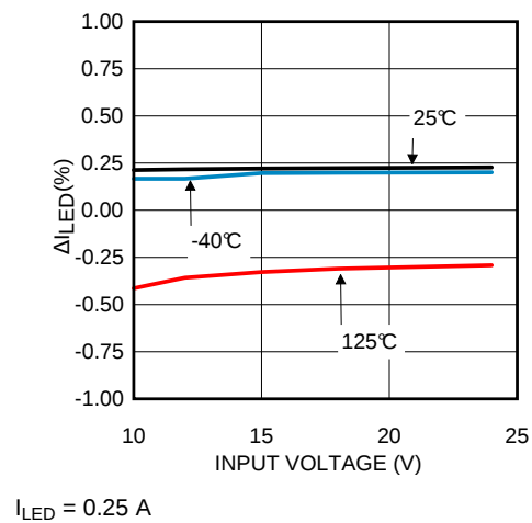
Figure 8. LED Current Regulation vs Input Voltage
