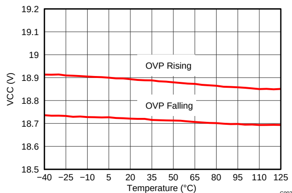
Figure 2. VCC OVP vs. Junction Temperature
