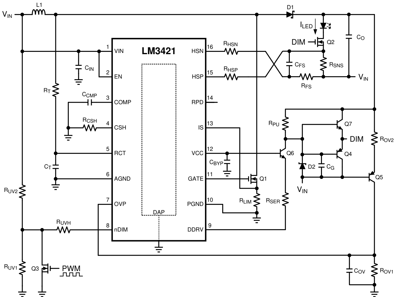
Figure 35. Buck-Boost Regulator
