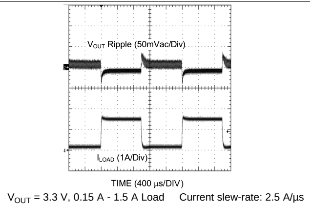
Figure 19. Load Transient
