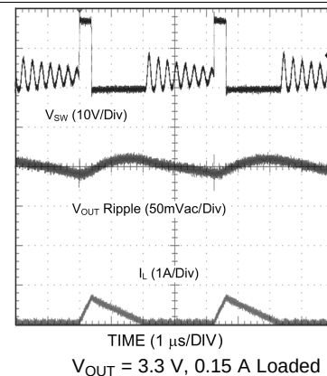
Figure 17. Discontinuous Mode Operation
