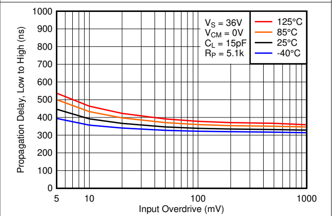
图 6-30. Low to High Propagation Delay vs. Input Overdrive Voltage, 36V
