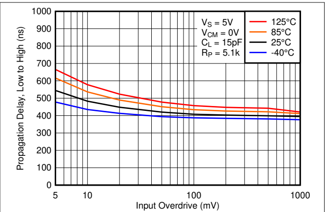
图 6-26. Low to High Propagation Delay vs. Input Overdrive Voltage, 5V
