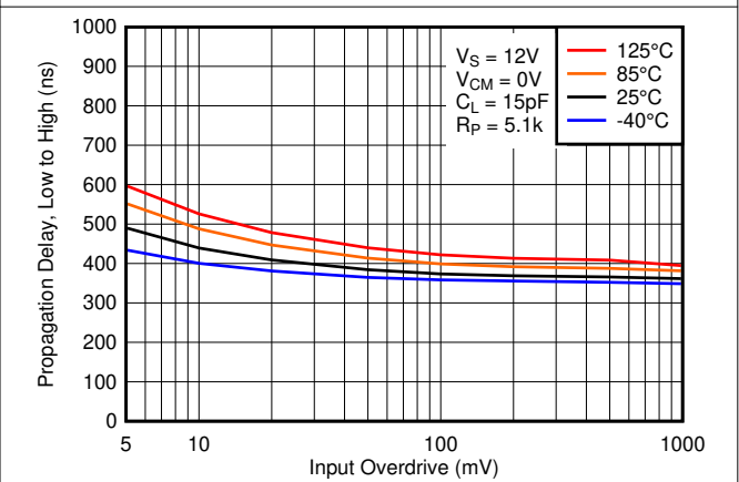
图 6-28. Low to High Propagation Delay vs. Input Overdrive Voltage, 12V
