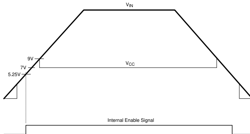
图 6-1. Vin and Vcc Sequencing
