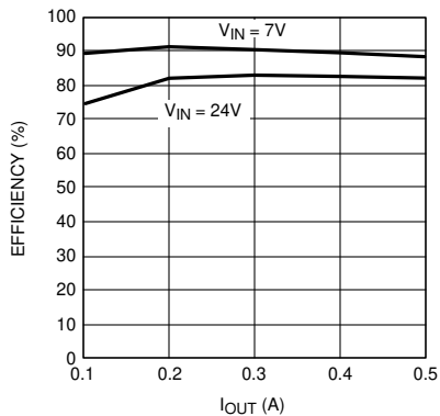
图 5-7. Demoboard Efficiency vs I_{OUT} and V_{IN}
