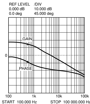
图 7-3. Gain and Phase of Modulator R_{\text{LOAD}} = 20 \text{ Ohms} and C_{\text{OUT}} = 22\mu\text{F}
