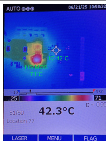
图 10-10. V_{\text{SUPPLY}} = 16\text{V} , I_{\text{LOAD}} = 20\text{A} , T_A = 25^\circ\text{C} , 无气流
