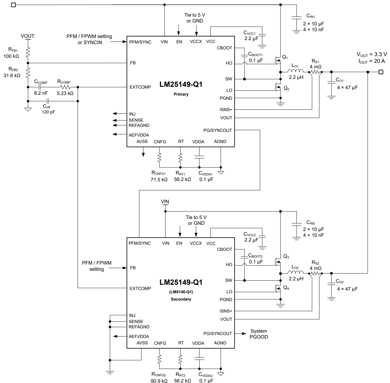
图 9-29. Application Circuit 3 With Two LM25149-Q1 Buck Controllers at 400 kHz
