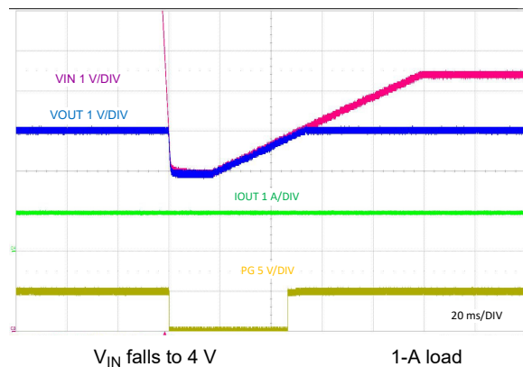
图 9-24. Line Transient Response to V_{IN} = 4 V
