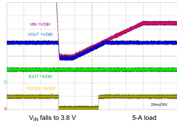
图 9-10. Cold-Crank Response to V IN = 3.8 V
