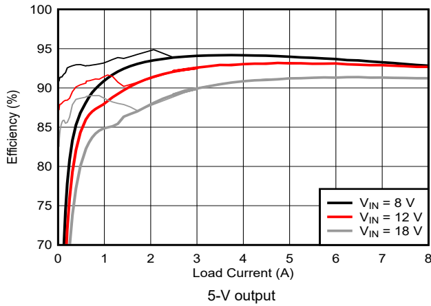
图 9-5. Efficiency vs I OUT
