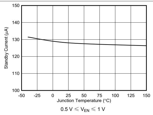
图 7-4. Standby Current vs. Temperature
