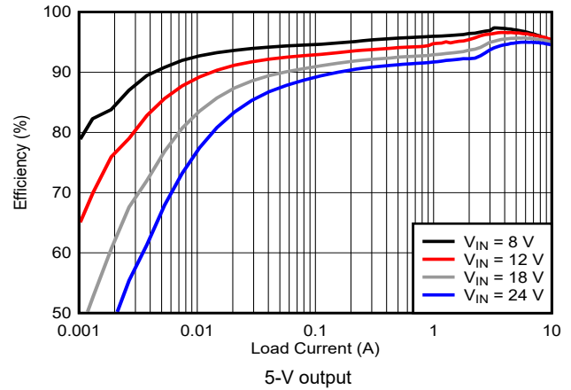
图 9-19. Efficiency vs I_{OUT} , Log Scale
