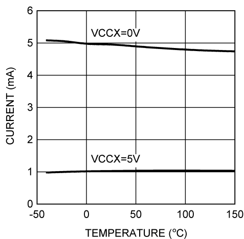
图 5-19. VIN Operating Current vs Temperature
