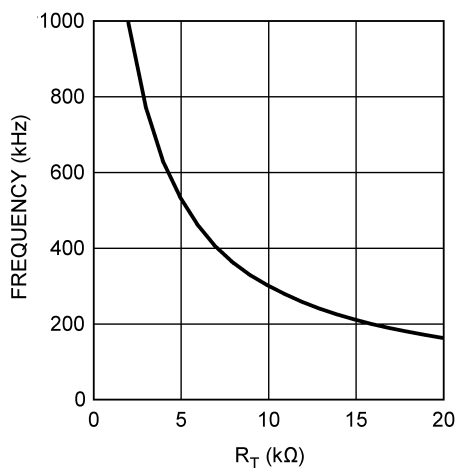
图 5-13. Frequency vs R_T
