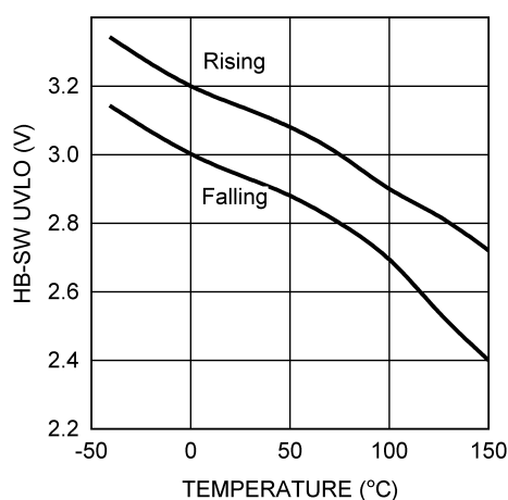
图 5-10. HB to SW UVLO vs Temperature
