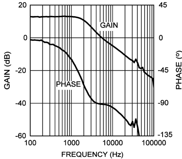
图 7-3. Modulator Gain and Phase
