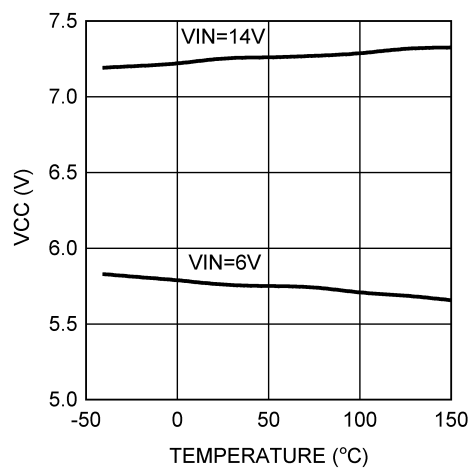
图 5-20. VCC vs Temperature
