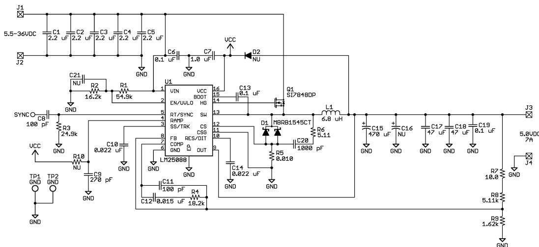
图 9-2. LM25088-2 Application Schematic
