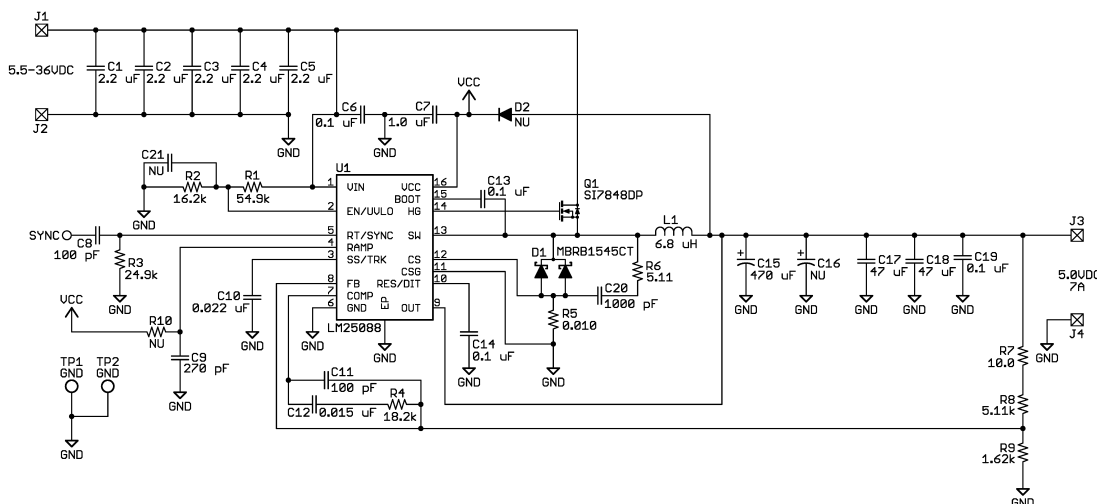
图 9-1. LM25088-1 Application Schematic
