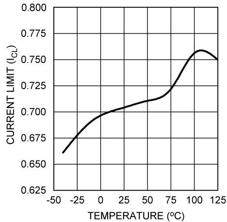
Figure 3. Current Limit vs Temperature
