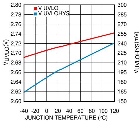
图 6-7. UVLO Threshold and Hysteresis vs Temperature
