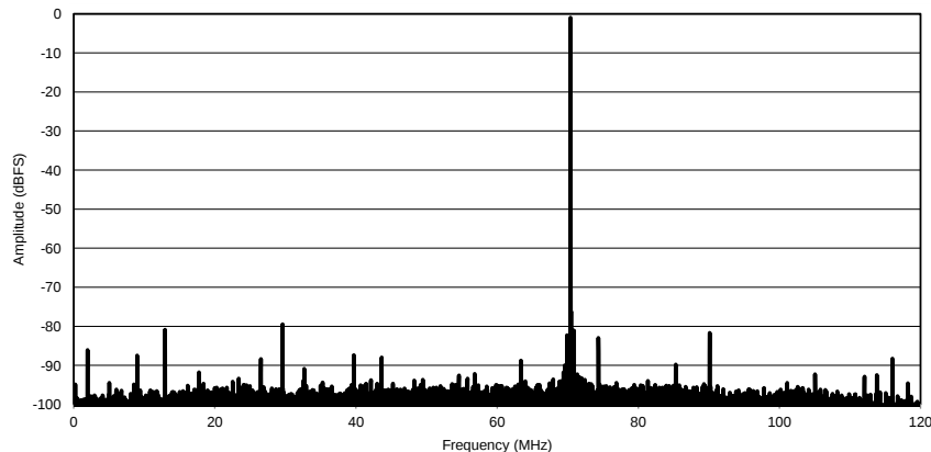
16 倍抽取率 — 频谱响应 f_S = 4\text{GHz} , F_{IN} = 1897\text{MHz} ( -1\text{dBFS} 时), f_{(NCO\_X)} = 1827\text{MHz}
