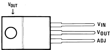
图 4-2. NDE Package, 3-Pin TO-220 (Front View)
