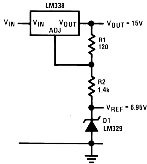
图 7-8. Regulator and Voltage Reference
