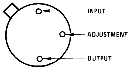
图 6-2. LM117H, LM117NDT NDT Package 3-Pin TO-39 (Metal Can) Bottom View
