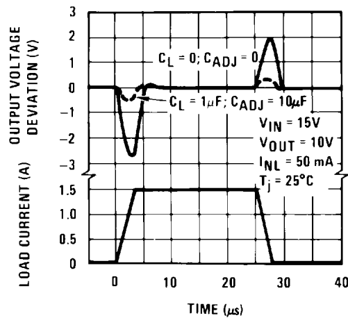
图 7-12. Load Transient Response
