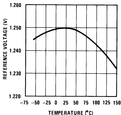
图 7-5. Temperature Stability
