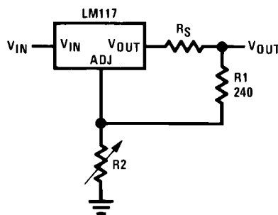
图 8-3. Regulator With Line Resistance in Output Lead
