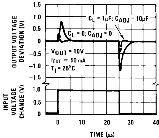
图 7-11. Line Transient Response
