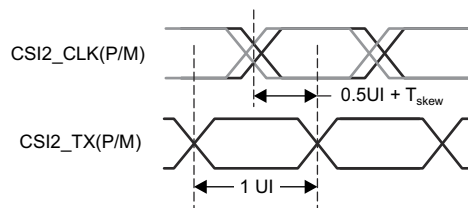
图 8-12. Clock and Data Timing in HS Transmission
