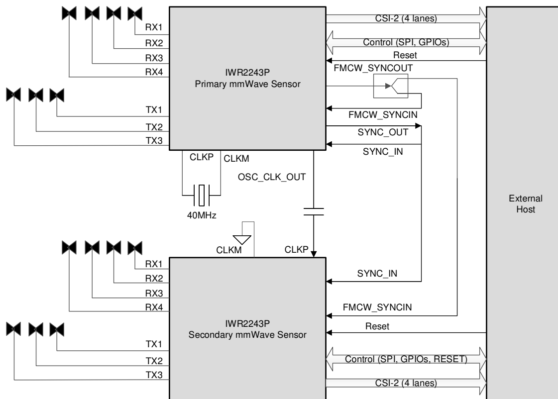
图 11-1. Imaging Radar using Cascade Configuration
