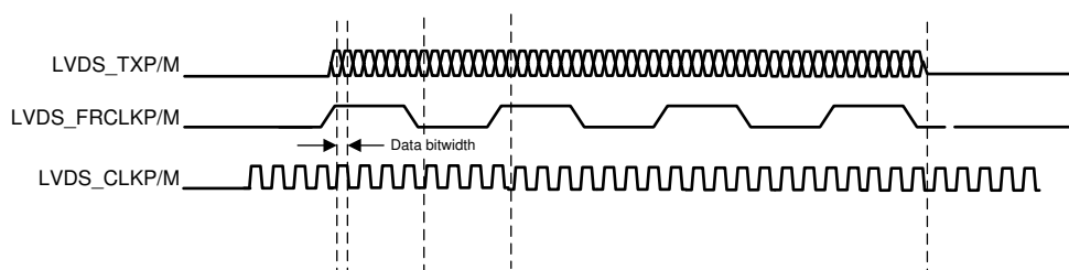
图 8-10. LVDS Interface Lane Configuration And Relative Timings
