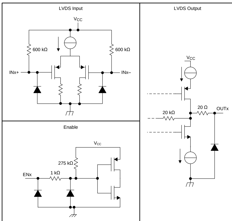
Figure 26. Device I/O Schematics
