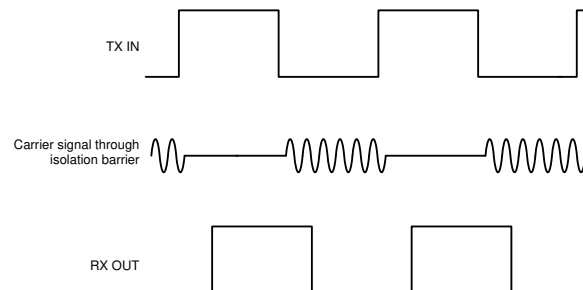
图 7-2. On-Off Keying (OOK) Based Modulation Scheme
