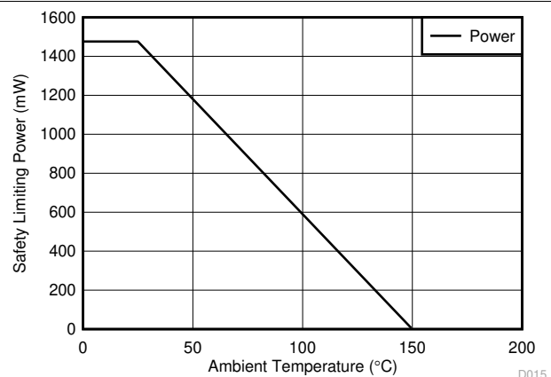
图 5-2. Thermal Derating Curve for Safety Limiting Power per VDE
