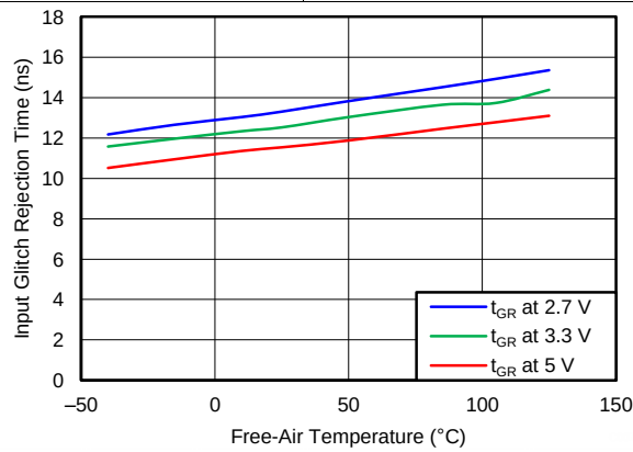
图 9. Input Glitch Rejection vs Free-Air Temperature
