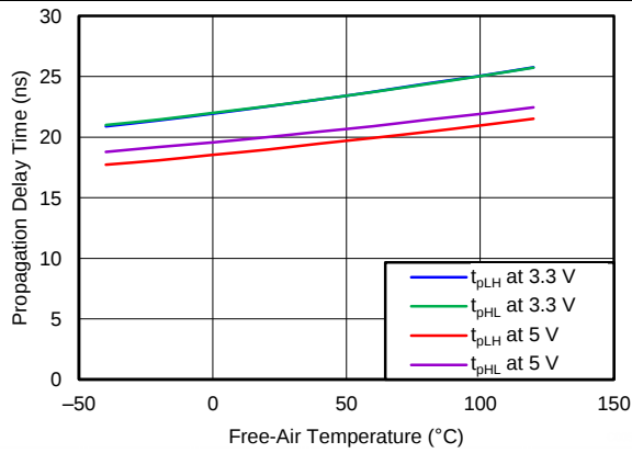
图 7. Propagation Delay Time vs Free-Air Temperature
