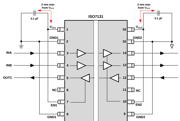
图 18. Typical ISO7131 Circuit Hook-up
