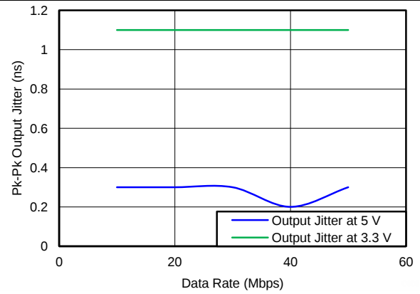
图 8. Output Jitter vs Data Rate
