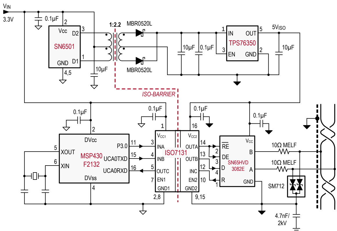
图 24. Isolated RS-485 Interface
