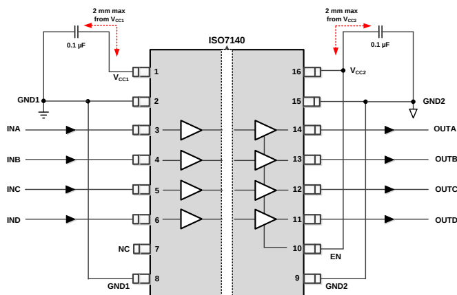
图 19. Typical ISO7140 Circuit Hook-up
