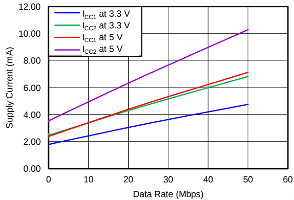
图 1. ISO7131 Supply Current for All Channels vs Data Rate
