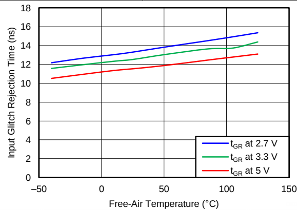
图 9. Input Glitch Rejection vs Free-Air Temperature
