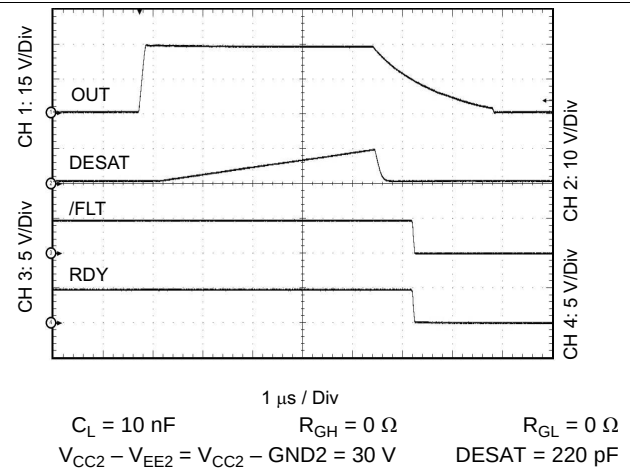
Figure 17. Output Transient Waveform DESAT, RDY, and \overline{\text{FLT}}
