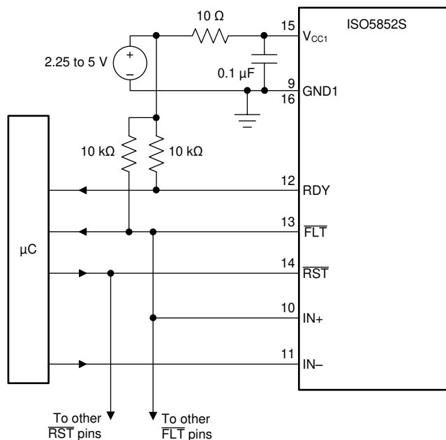
图 10-6. Global Shutdown With Inverting Input Configuration
