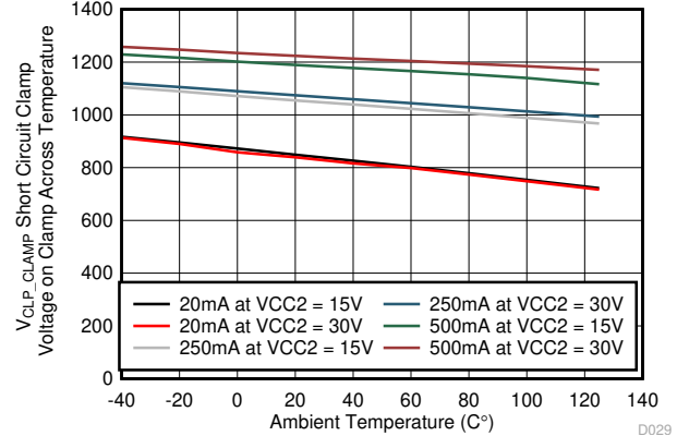
图 7-40. V_{CLP\_CLAMP} - Short-Circuit Clamp Voltage on CLAMP Across Temperature
