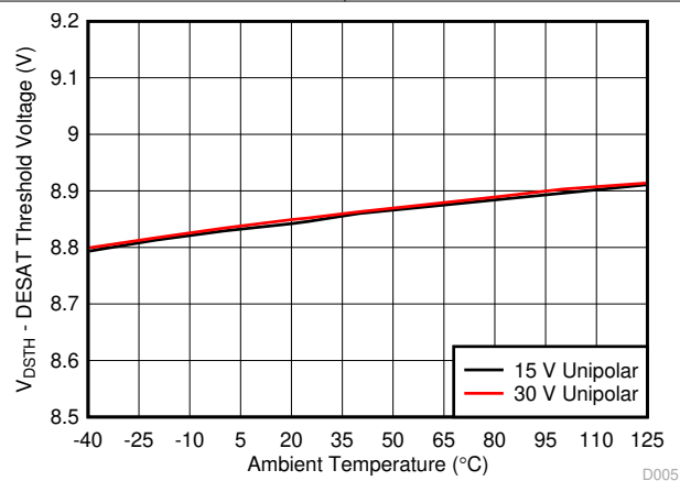
Unipolar: V_{CC2} - V_{EE2} = V_{CC2} - \text{GND2} 图 7-8. DESAT Threshold Voltage vs Temperature
