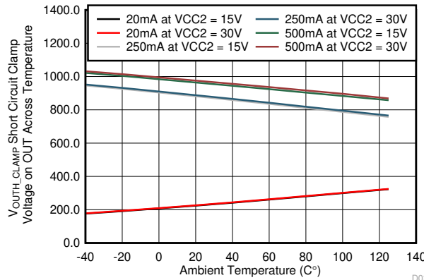
图 7-41. V_{OUTH\_CLAMP} - Short-Circuit Clamp Voltage on OUTH Across Temperature
