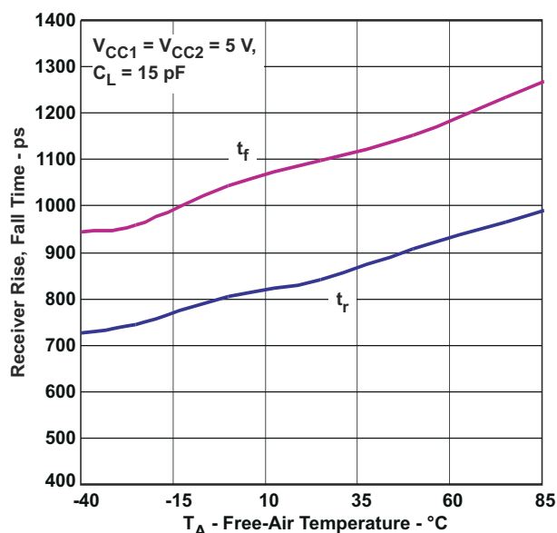
图 6-10. Receiver Rise, Fall Time vs Free-Air Temperature
