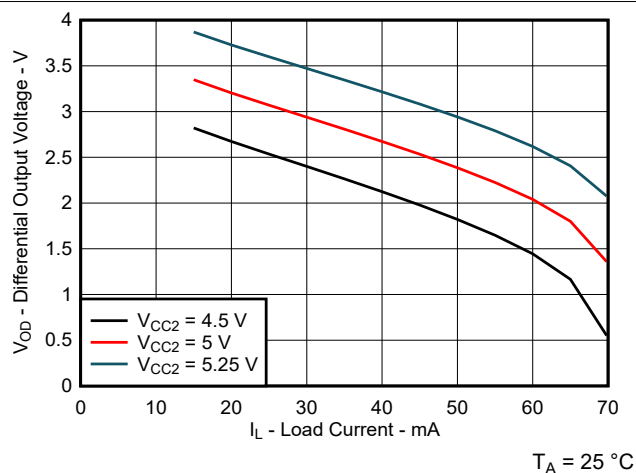
图 6-12. Driver Differential Output Voltage vs Load Current
