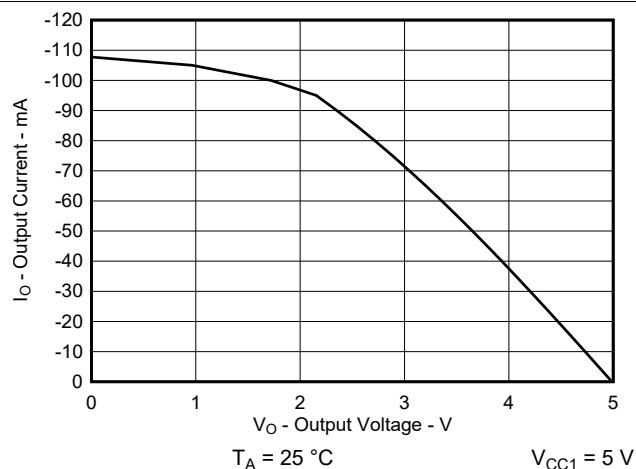
图 6-13. Receiver High-Level Output Current vs High-Level Output Voltage
