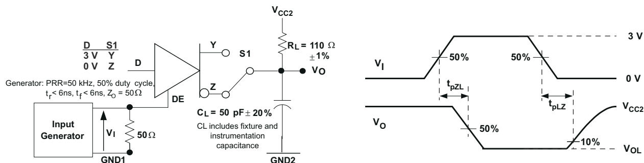
图 7-6. Driver Low-Level Output Enable and Disable Time Test Circuit and Voltage Waveform
