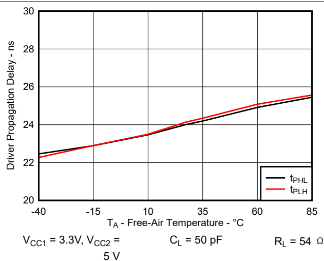
图 6-5. Driver Propagation Delay vs Free-Air Temperature
