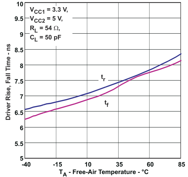
图 6-9. Driver Rise, Fall Time vs Free-Air Temperature
