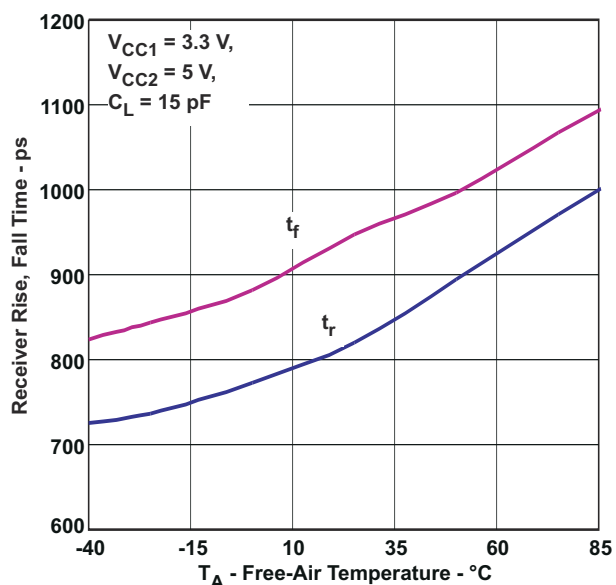
图 6-11. Receiver Rise, Fall Time vs Free-Air Temperature
