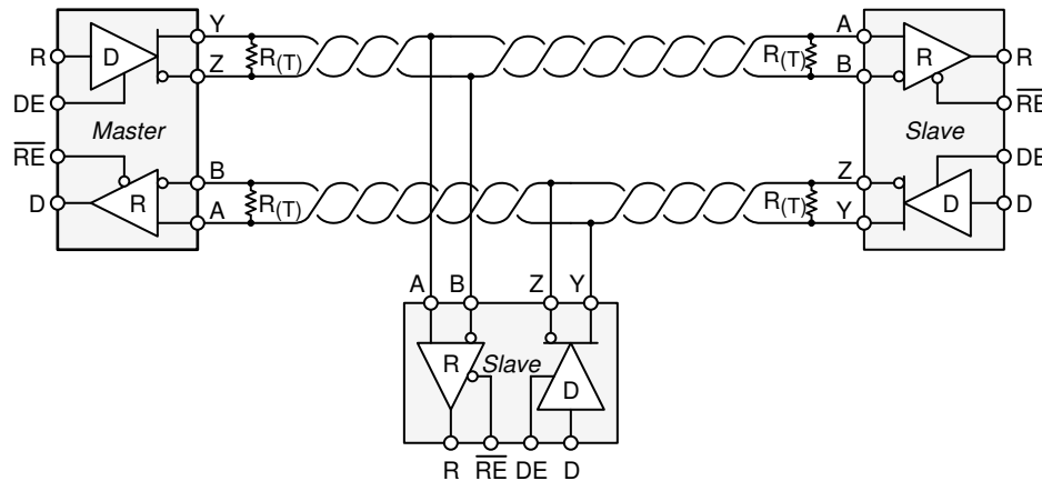
图 9-1. Half-Duplex Transceiver Configurations
