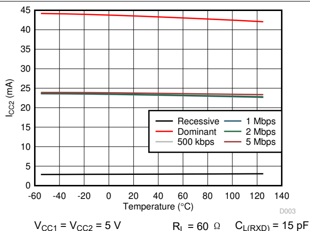
图 6-7. I_{CC2} vs Ambient Temperature for Recessive, Dominant and Different CAN Datarates
