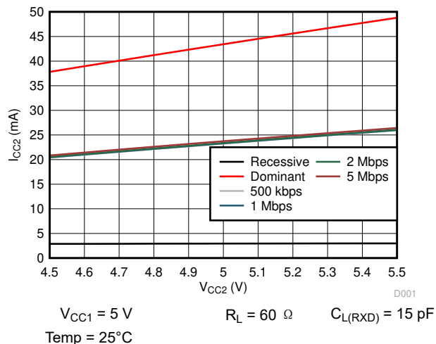
图 6-5. I_{CC2} vs V_{CC2} for Recessive, Dominant and Different CAN Datarates
