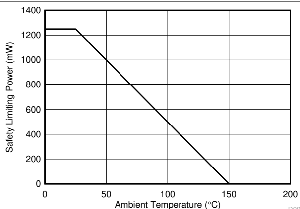
图 6-4. Thermal Derating Curve for Limiting Power per VDE for DWV-8 Package
