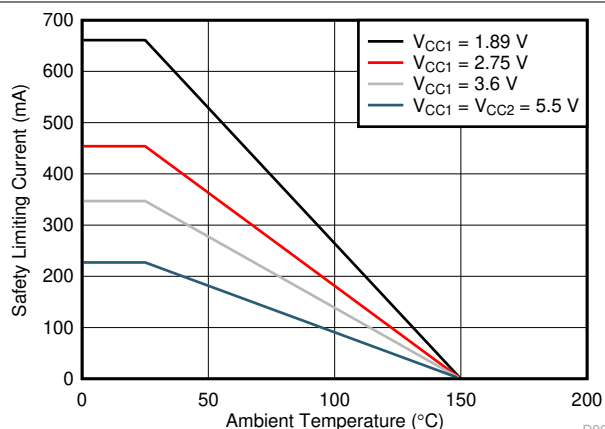
图 6-2. Thermal Derating Curve for Limiting Current per VDE for DWV-8 Package
