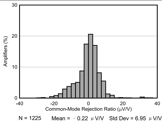
图 7-8. Typical CMRR Distribution
