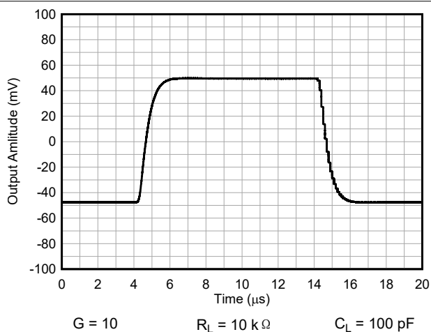
图 7-30. Small-Signal Response
