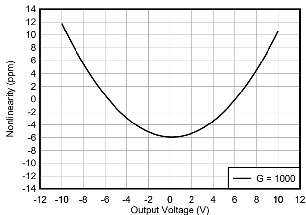
图 7-40. Gain Nonlinearity
