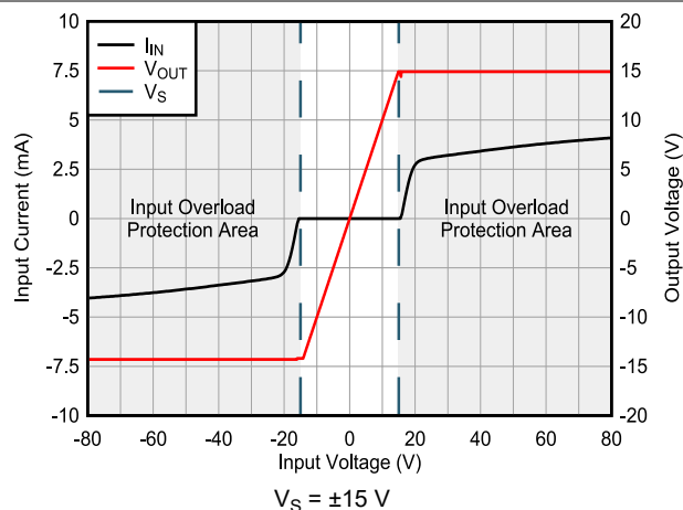
图 7-38. Input Current vs Input Overvoltage
