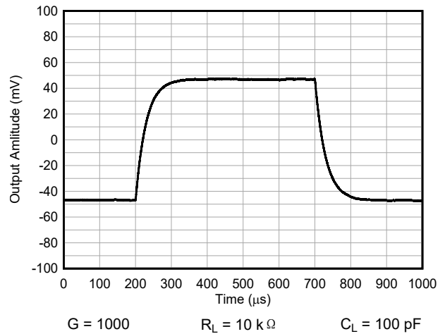
图 7-32. Small-Signal Response
