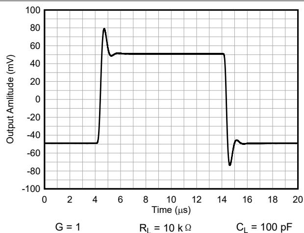
图 7-29. Small-Signal Response
