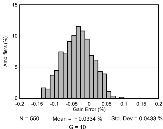
图 7-10. Typical Gain Error Distribution
