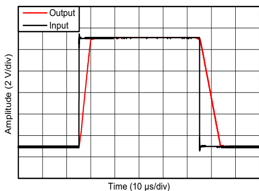
图 45. Small-Signal Response
