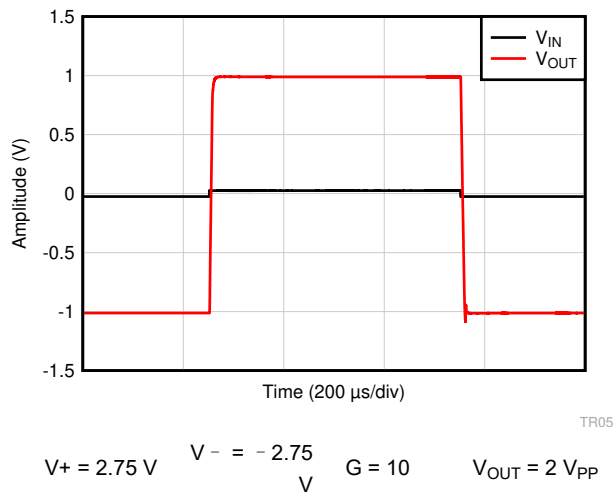
图 6-47. Large Signal Step Response
