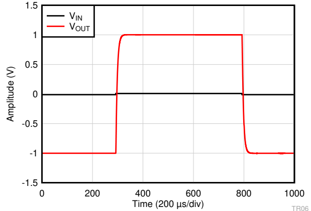
图 6-50. Large Signal Step Response
