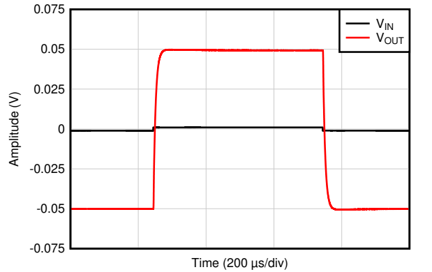
图 6-50. Large Signal Step Response
