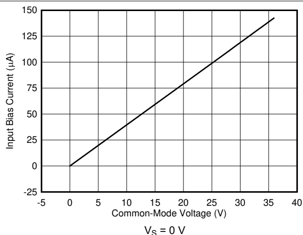
图 6-18. Input Bias Current vs. Common-Mode Voltage
