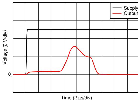
图 6-26. Start-Up Response
