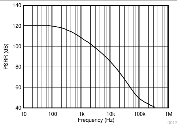
图 6-12. Power-Supply Rejection Ratio vs Frequency
