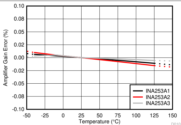
图 6-10. Amplifier Gain Error vs Temperature
