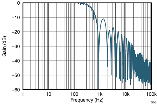
图 6-1. Frequency Response
