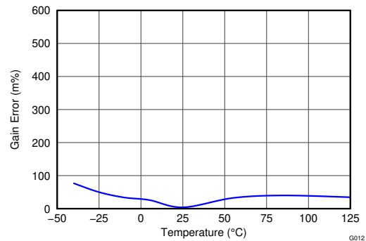
图 6-6. Shunt Input Gain Error vs. Temperature
