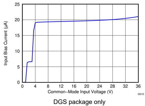
图 6-12. Input Bias Current ( I_{B+} + I_{B-} ) vs. Common-Mode Voltage DGS package only
