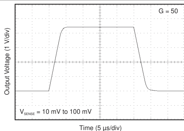
图 6-17. Step Response
