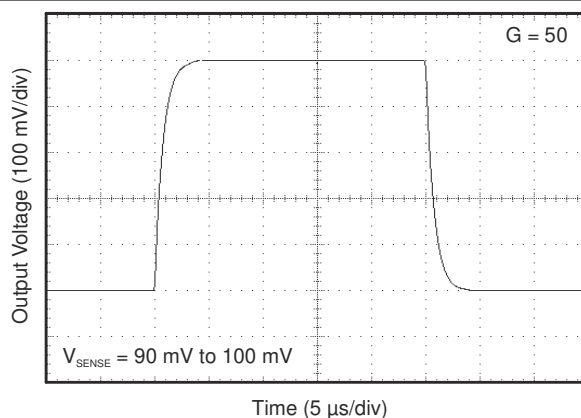
图 6-18. Step Response
