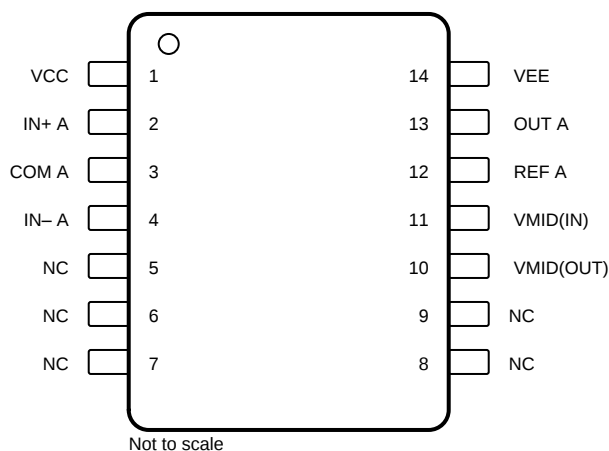
Pin Functions
