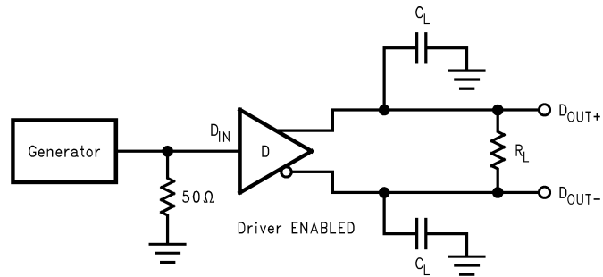
Figure 19. Driver Propagation Delay and Transition Time Test Circuit
