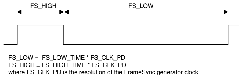
图 7-14. Internal FrameSync Signal
