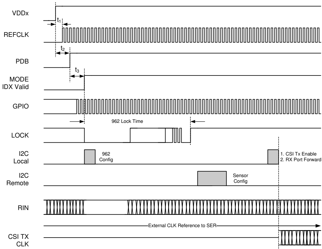
图 8-16. Power-Up Sequencing With Non-Synchronous Clocking Mode
