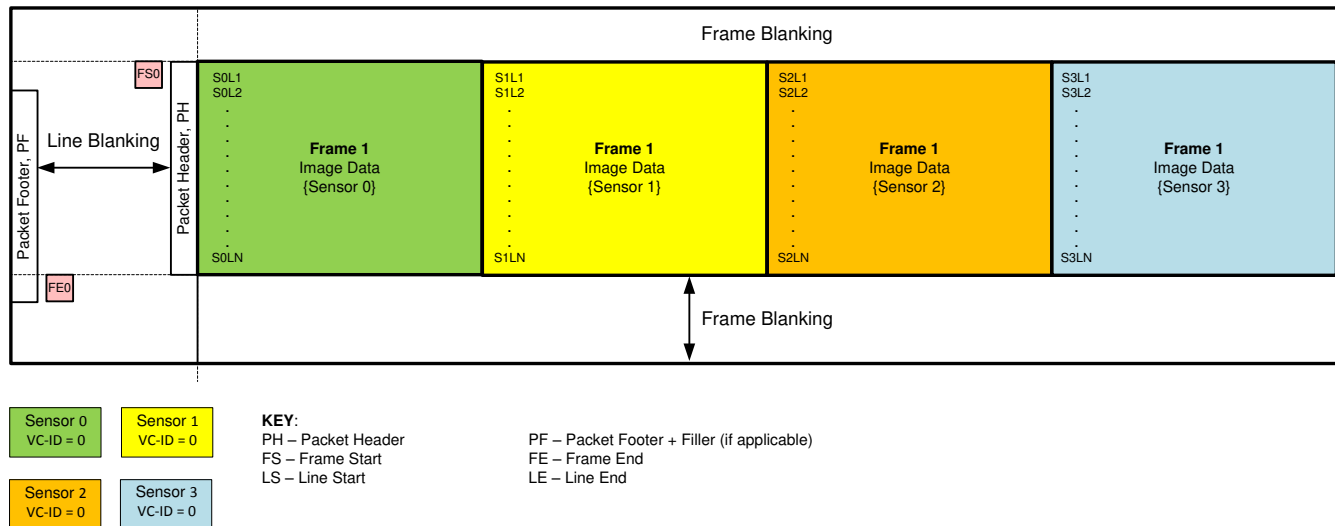
图 7-17. Line-Concatenated Format
