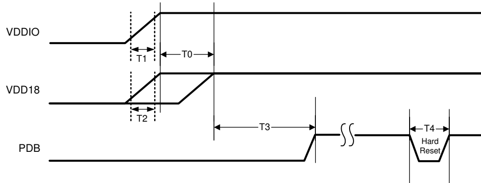
图 6-11. Power-Up Sequencing
