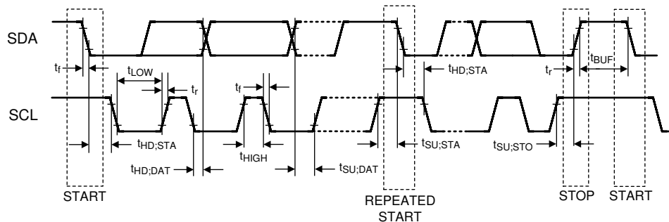
图 5-10. Basic Operation
