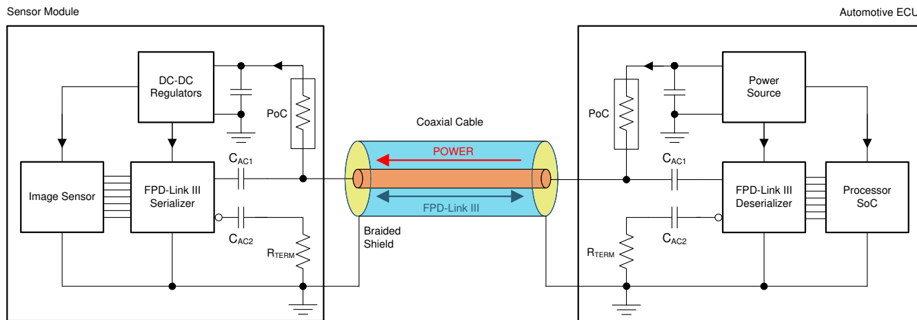
图 6-1. Power Over Coax (PoC) System Diagram
