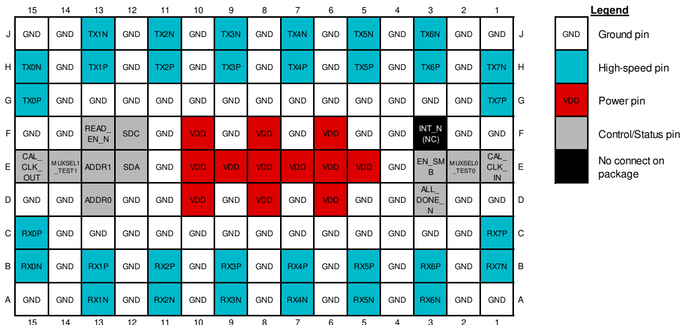
Figure 6-1. Top View
