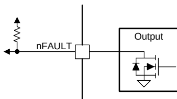
Figure 17. nFAULT Pin
