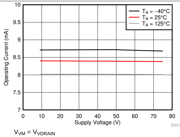
图 2. VM Supply Current Over Supply Voltage
