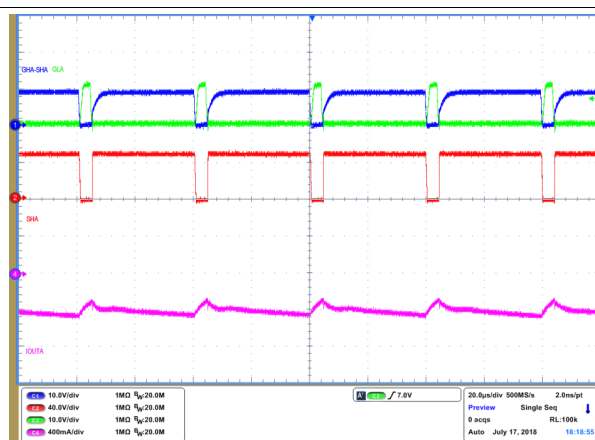
图 65. Gate Driver Operation 90% Duty Cycle
