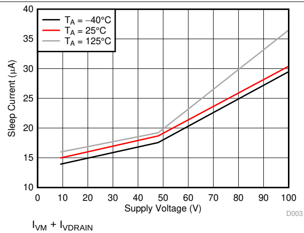
图 4. Sleep Current Over Supply Voltage
