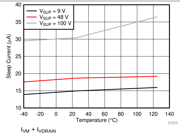
图 5. Sleep Current Over Temperature
