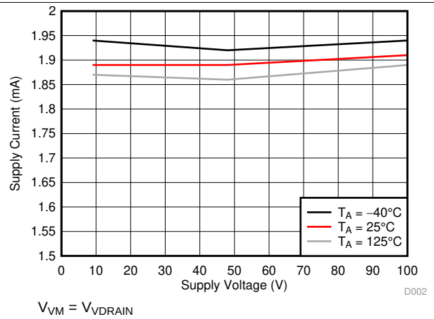
图 3. V DRAIN Supply Current Over Supply Voltage
