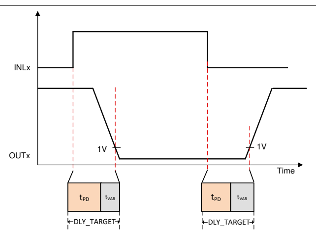
图 8-21. Delay Compensation with current flowing into the phase
