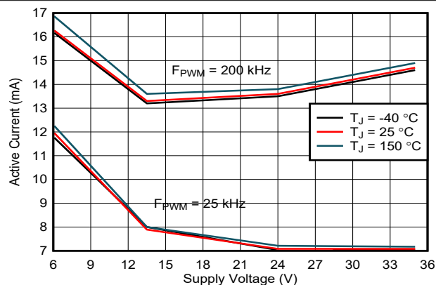
图 7-2. Supply current over supply voltage
