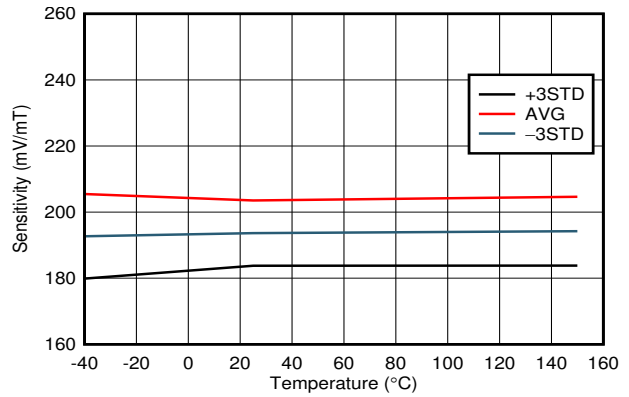
DRV5056Z1, V_{CC} = 5.0V
