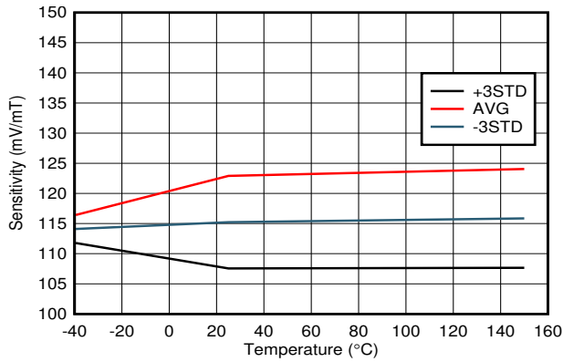
DRV5056Z1, V_{CC} = 3.3V
