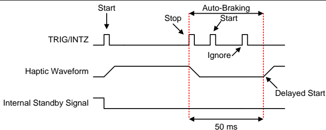
图 43. Trigger-Pulse and Delayed Start with Ignored Pulse (RTP or Waveform Sequencer)
