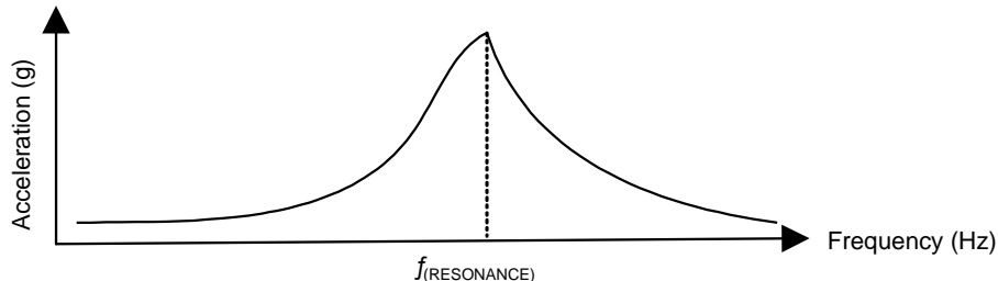
图 101. Typical LRA Response
